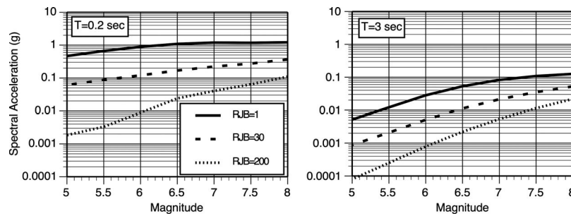
Figure 9. Magnitude scaling for strike-slip earthquakes and rock site condition ( V_{S30}=760 m/s) for T=0.2 sec and T=3 sec.
