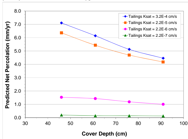
Figure 8. Predicted Net Percolation with Different Cover Material Depths and Tailings Saturated Hydraulic Conductivity (Ksat)
