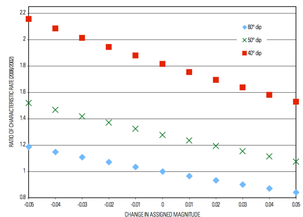
Figure J-1. Plot of the ratio (2008/2002 hazard maps) of rate of characteristic earthquakes resulting from rounding characteristic magnitude (M) to two decimal places and alternative fault-dip models.
