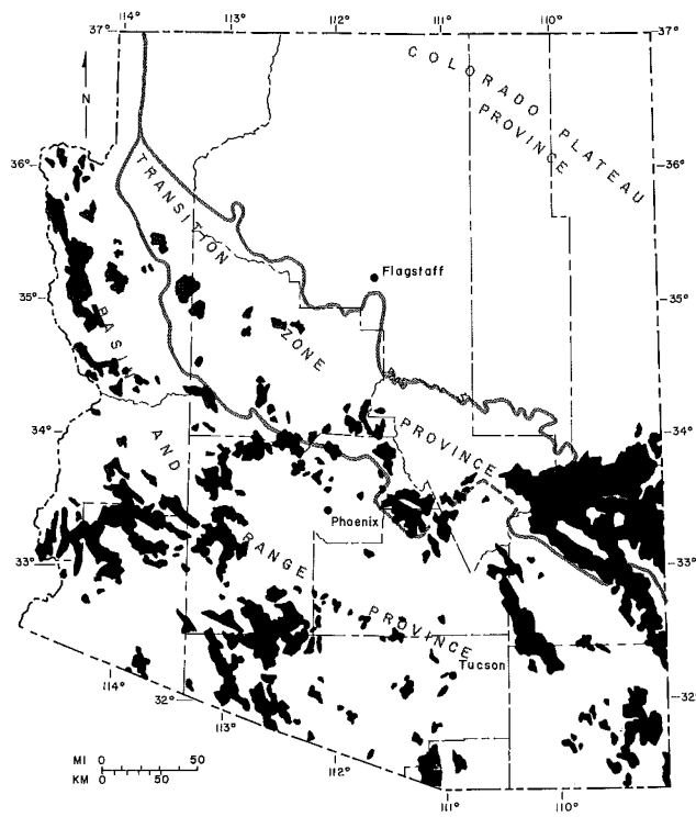
DISTRIBUTION OF MID-TERTIARY (40-15 m.y.) VOLCANIC ROCKS
