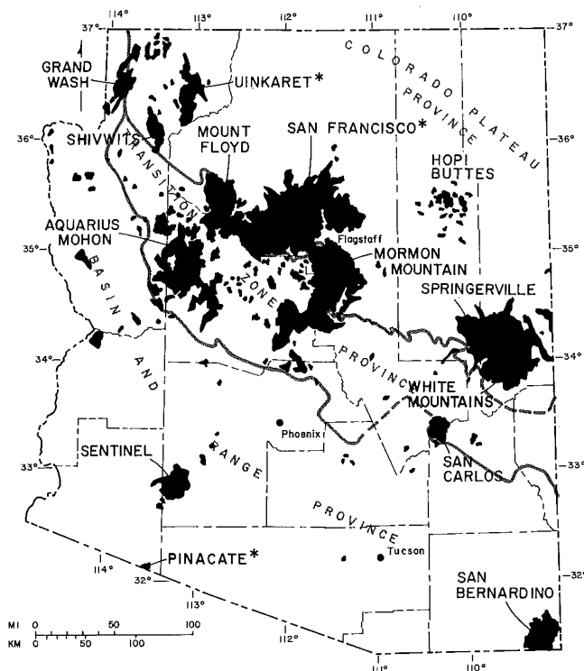
DISTRIBUTION OF UPPER CENOZOIC (15-0 m.y.) VOLCANIC ROCKS AND VOLCANIC FIELDS
