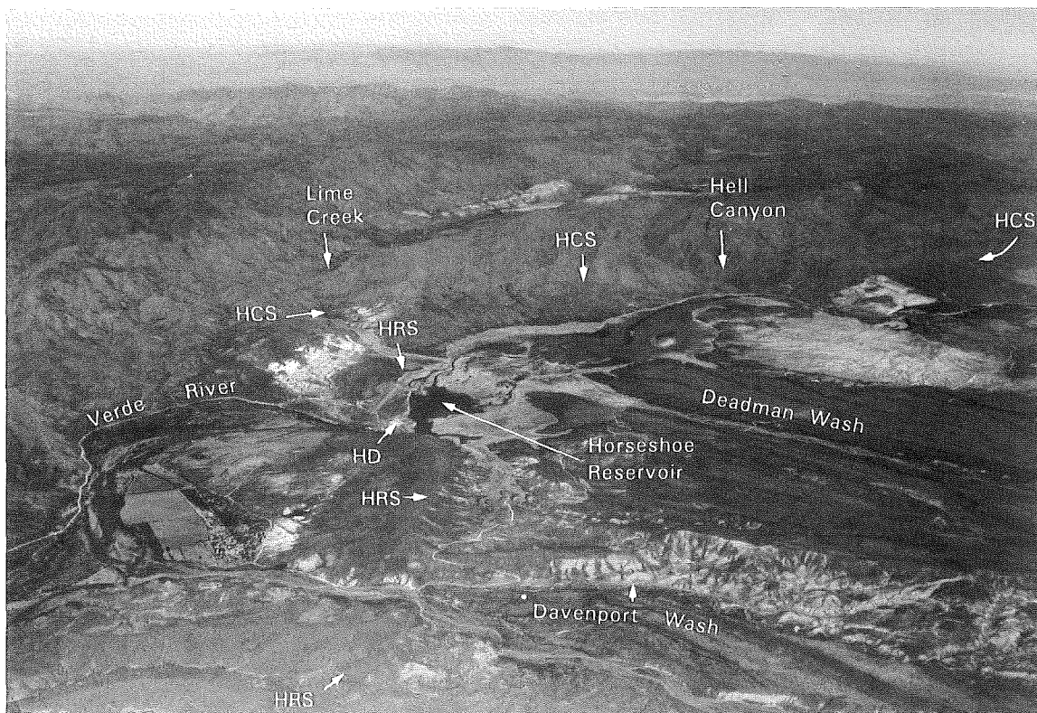
Figure 4. Aerial view toward the northwest of the two segments of the Horseshoe fault. The Hell Canyon segment (HCS) trends along the range in the middle ground. The Horseshoe Reservoir segment (HRS) trends away from the viewer toward the Hell Canyon segment. Horseshoe Dam (HD) is partially concealed in the middle ground.
