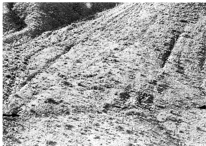
Figure 6. Aerial view toward the west of a linear east-facing scarp (between arrows) along the Hell Canyon segment of the Horseshoe fault between Lime Creek and Hell Canyon (Figures 3 and 5). The displacement of the alluvial-fan surface across this scarp is about 2 meters. The slope of the alluvial-fan surface is 10° to 13°; the maximum slope of the scarp is about 27°.
