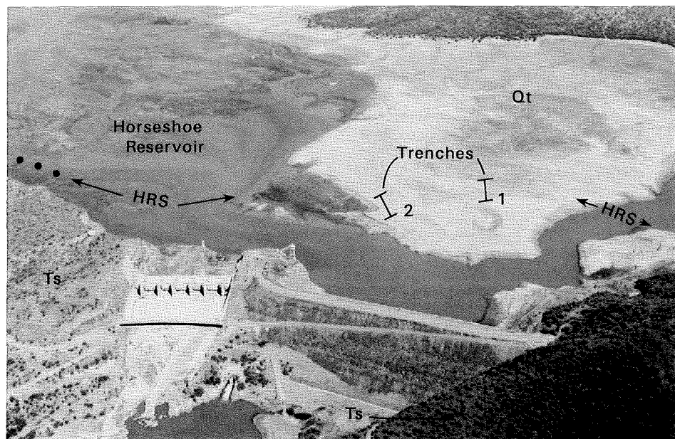
Figure 1. Aerial view of Horseshoe Dam (foreground). This view toward the north-northwest shows the curving north-facing scarp on the terrace surface (Qt) along the Horseshoe Reservoir segment (HRS) of the Horseshoe fault, a segment that was only recently identified. The approximate locations of two trenches excavated across this scarp are shown. (See section titled "Horseshoe Reservoir Segment.") Ts indicates tuffaceous sedimentary and volcanic rocks of late Tertiary age (Figure 3).
