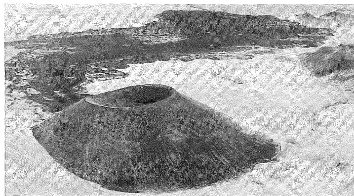
Figure 2. Aerial photograph of SP Crater and basalt flow. Photo by Dale Nations.
