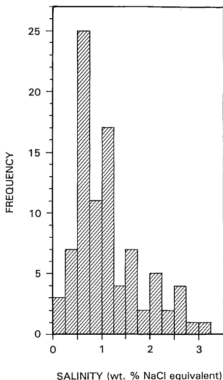
Figure 4. Histogram of fluid-inclusion salinities from vein deposits in the Artillery manganese district. Samples are from the Shannon mine area (33 inclusions in calcite), Priceless mine area (43 inclusions in barite and 4 in chalcedonic quartz), and Black Diamond mine (9 inclusions in calcite). Analyses by J.T. Duncan (unpublished data) and Spencer and others (1989a).
