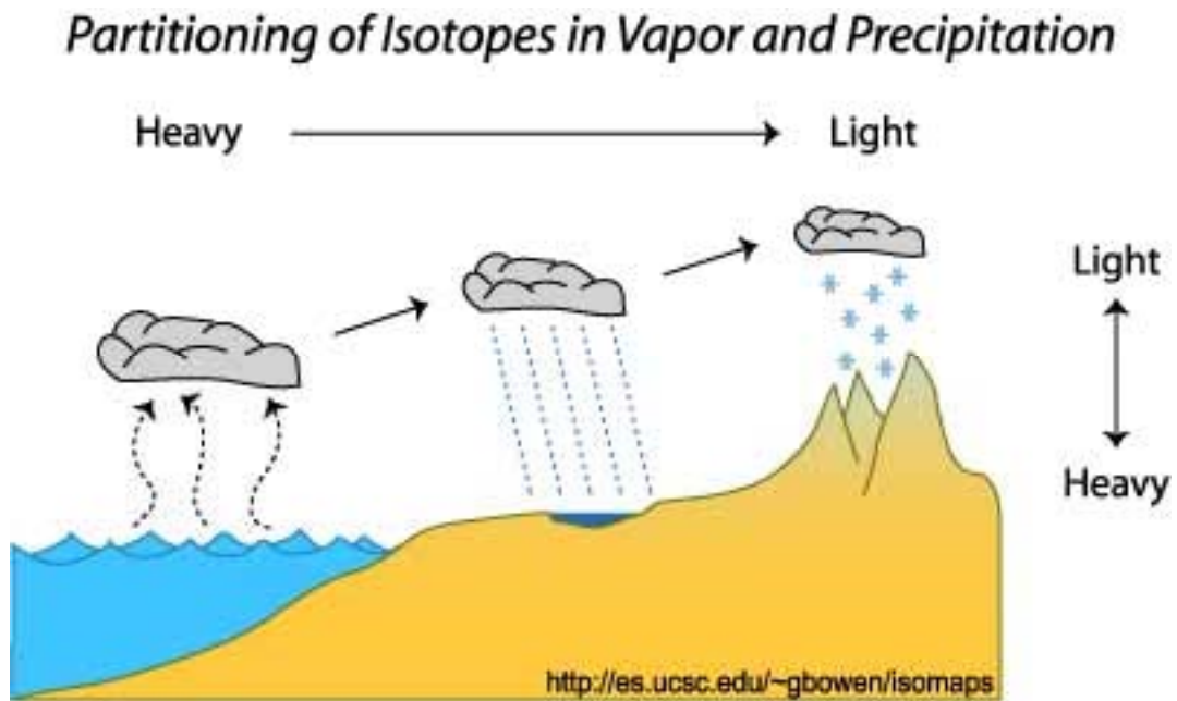
Fig. 12. Altitude and Continental Effect for \delta^{18}\text{O} . Obtained from Bowen, 2004.
