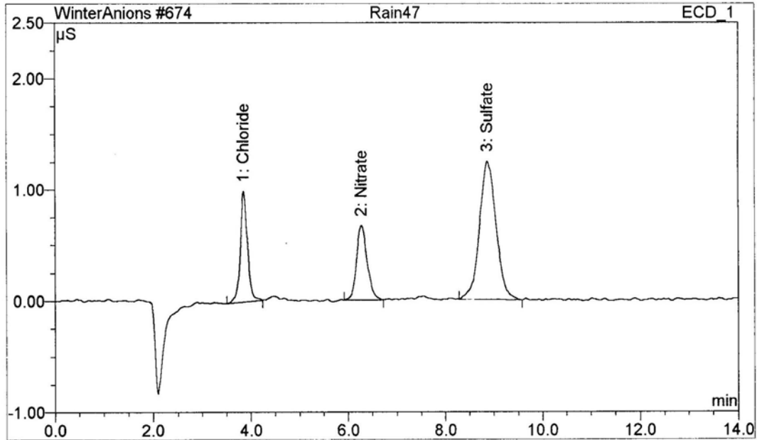
Fig. 3 Sample readoff from the Ion Chromatograph.
