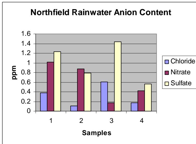
Fig. 10 Rainwater collected in Northfield, MN from 10/1/04 to 10/11/04.
