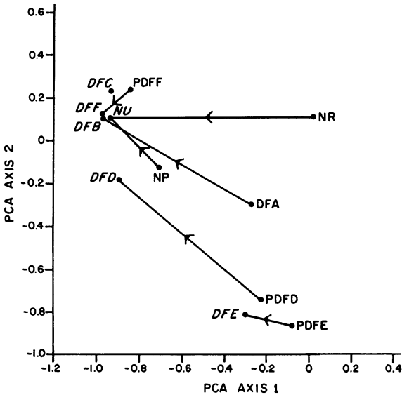
FIG. 3. Principal components analysis (PCA) ordination of cover data from Coleogyne communities in the Panamint Mountains. Paired disturbed/undisturbed sites are linked with arrows pointing toward the undisturbed site. Sites are Wood Canyon: DFA-DFF (debris flows A–F), PDFD-PDFF (pipeline corridors across debris flows D–F); and Nemo Crest: NP (pipeline corridor), NR (abandoned road), and NU (undisturbed hillslope).
