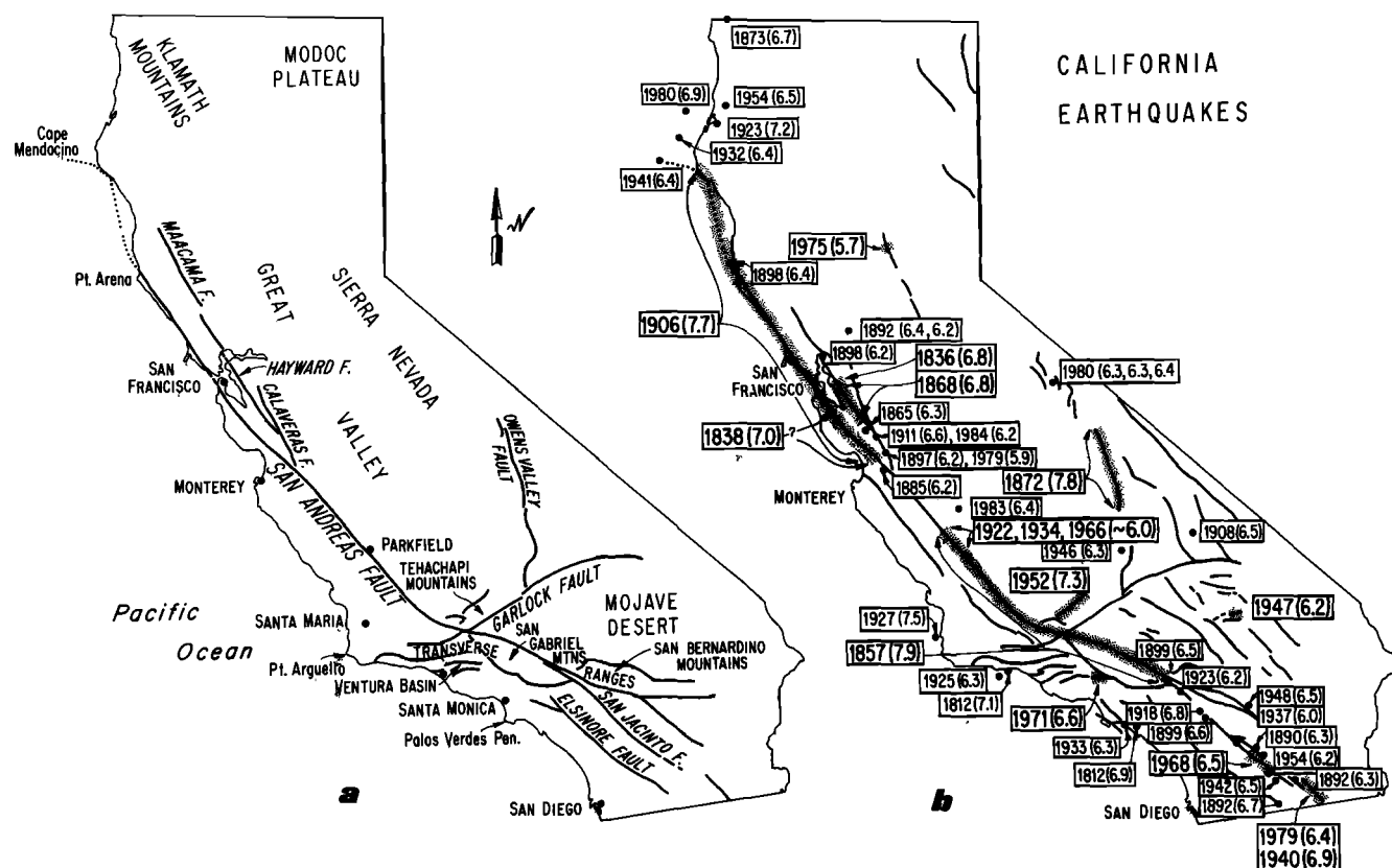
Fig. 1. (a) Major active faults, physiographic features, and (b) locations of historically recorded moderate to large earthquakes that have occurred in California. Faults that have produced coseismic surface ruptures are stippled. Onshore and offshore events of M \geq 6.2 are listed in Tables 1 and 3, respectively.
