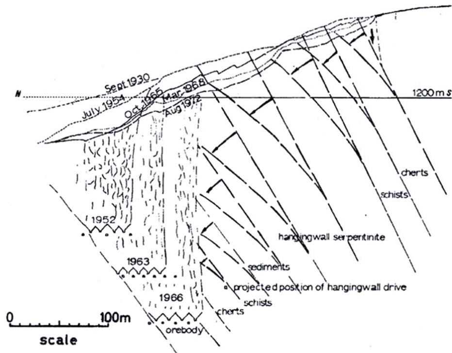
FIG 2 SECTION THROUGH THE HAVELOCK SUBSIDENCE ZONE Illustrating the development of the subsidence zone by tilting towards the mining.
