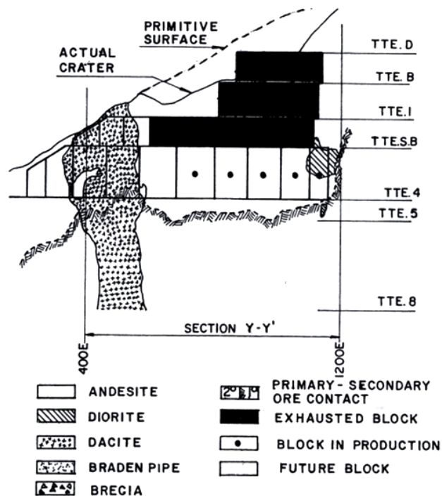
FIGURE 5. Geology and Blocks. North Mine Cross Section
