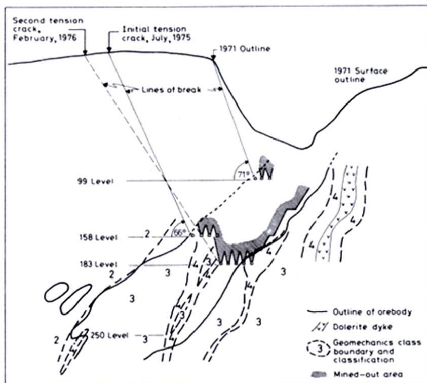
Fig. 2 Section through orebody, 620 section
