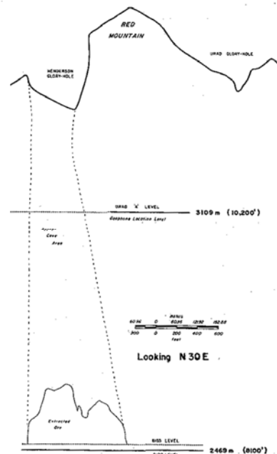
Figure 20. Cross section of Urad and Henderson mines.
