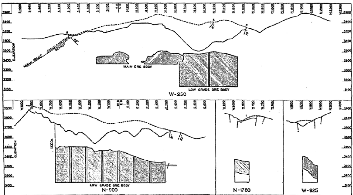
FIG. 3.—SECTIONS THROUGH OREBODY SHOWING STOPED AREAS AND RESULTING SURFACE SUBSIDENCE.
