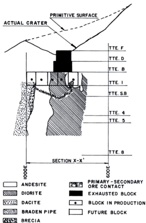
FIGURE 4. Geology and Blocks. South Mine Cross Section
