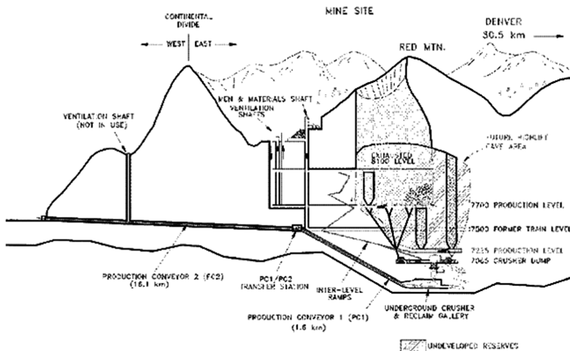
FIG 1 - General cross-section of the Henderson Mine and Mill.
