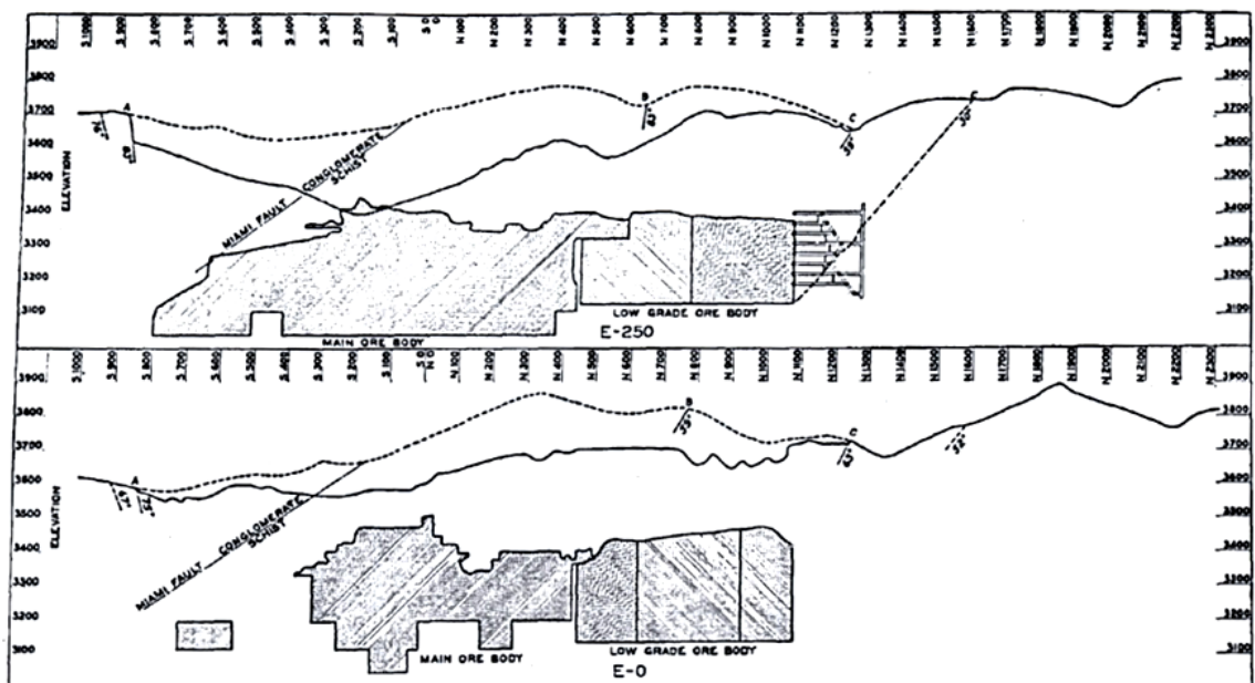
FIG. 2.—SECTIONS THROUGH OREBODY SHOWING STOPED AREAS AND RESULTING SURFACE SUBSIDENCE.
