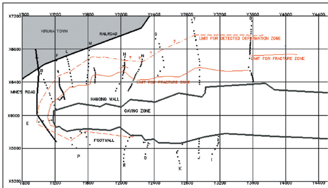
Fig. 1. Location of the caving, fracture, and deformation zones in 2000 and benchmark line networks (black points) at Kiruna mine.
