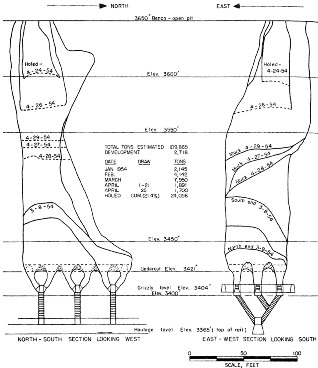
FIGURE 8. - Section Through Transfer Block.
