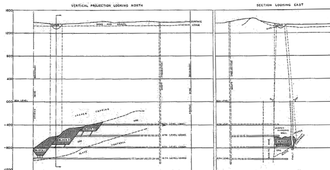
FIG. 1.—MINING SYSTEM AND RESULTING SUBSIDENCE, ATHENS MINE.
