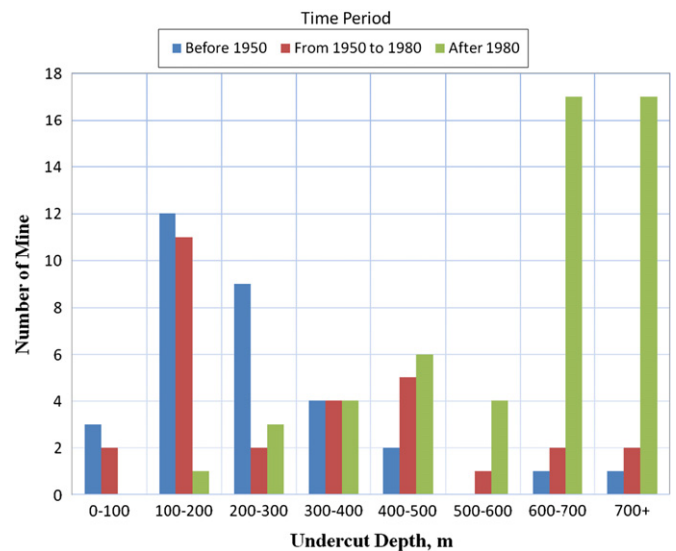
Fig. 5. Breakdown of undercut depths associated with the block caving cases in the database, showing a trend towards the development of deeper undercuts.
