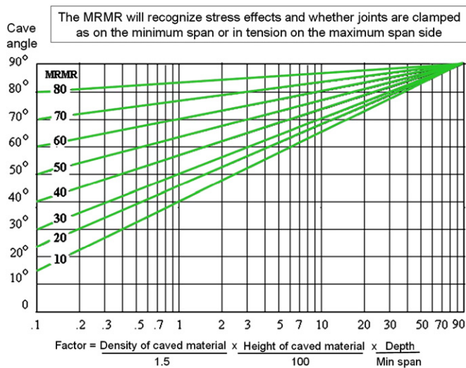
Fig. 1. Laubscher's empirical design chart for assessing cave angle (angle of break) as a function of mining rock mass rating (MRMR) value and the height and depth of the caved block (after [1]).
