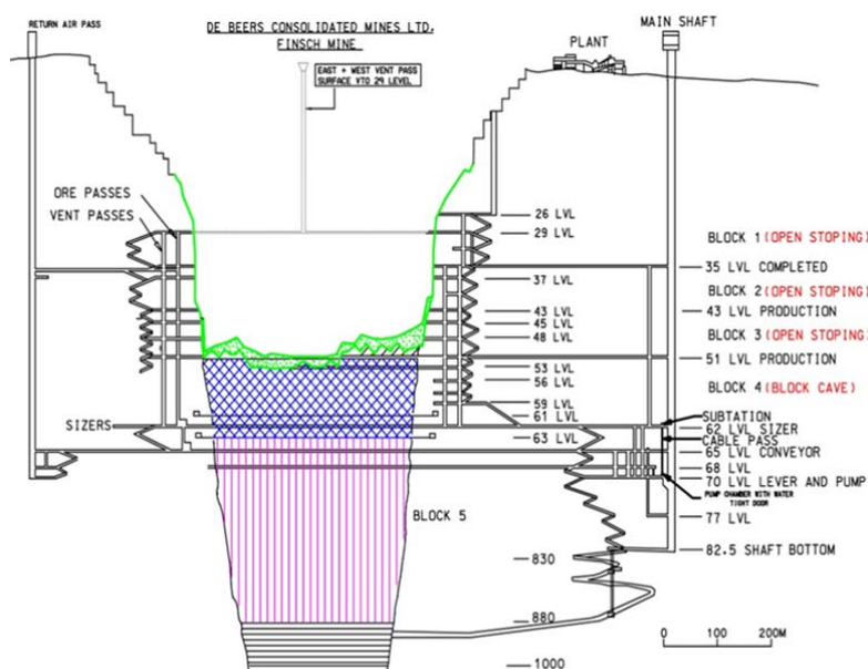
Fig. 2 Section through Finsch Mine showing mining blocks
