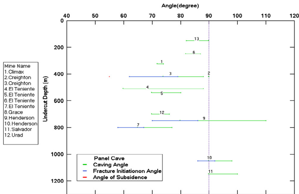
Fig. 9. Undercut depth versus caving, fracture initiation and subsidence angles for panel caving operations. Each line segment represents the range in angles measured from different from sides of the undercut; the greater the range the higher the degree of asymmetry.
