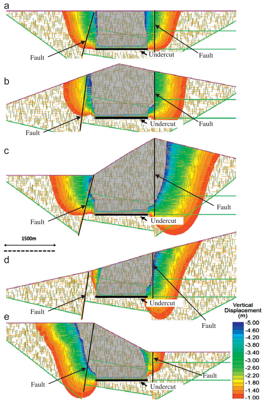
Fig. 12. Finite-element modeling of influence of topography on caving-induced subsidence assuming typical surface profiles visually identified in the UBC database. The same geological inputs used for the comparative models in Chapter 3 were applied. In order of increasing degree of asymmetry (cave–surface interactions) relative to the position of the undercut below, these are: (a) flat topography, (b) mountain peak, (c) rising slope ending in a mountain peak, (d) rising slope, and (e) slope with plateau. Note that gray shaded area approximates zone of caving. (For interpretation of the references to color in this figure caption, the reader is referred to the web version of this article.)
