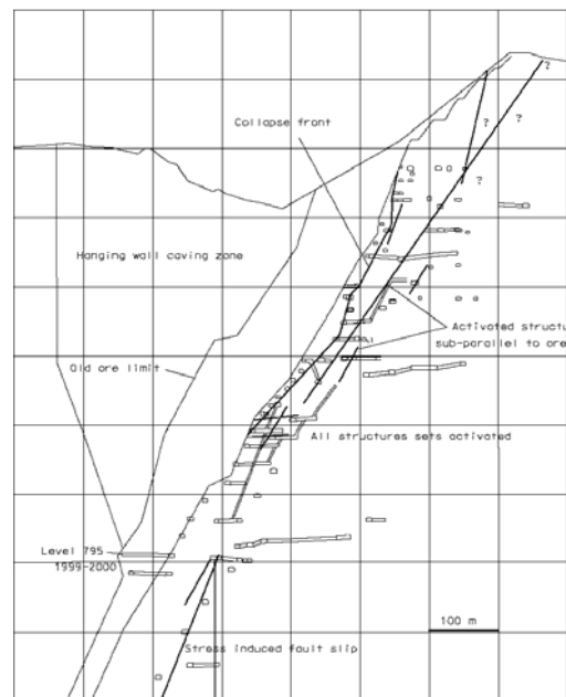
Fig 3 - Mapped failure on section Y23 until year 2000.
