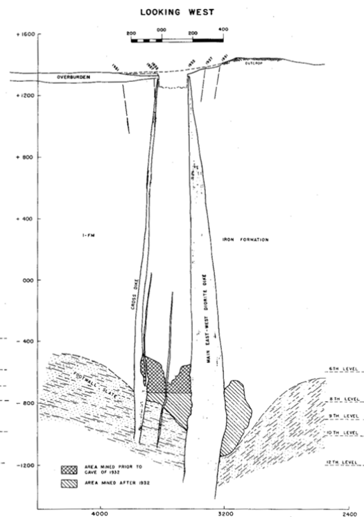
Fig. 30. Athens Mine, north-south cross section.
