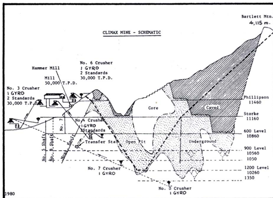
Figure 32. General Mine Layout-Schematic
