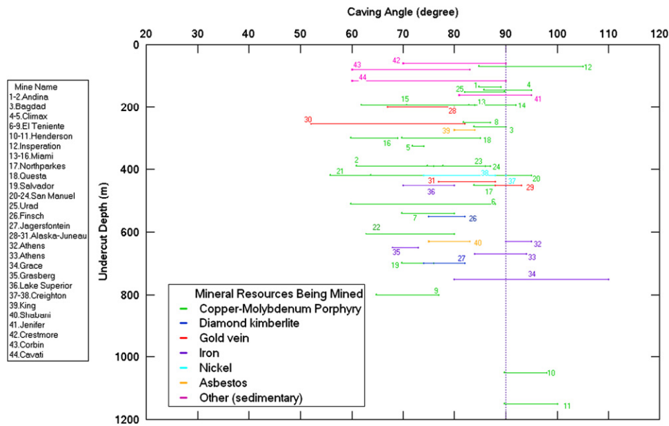
Fig. 13. Undercut depth versus caving angle for global block and panel caving operations, color coded according to the resource being mined. Each line segment represents the range in caving angles measured from different sides of the undercut; the greater the range the higher the degree of asymmetry. (For interpretation of the references to color in this figure caption, the reader is referred to the web version of this article.)
