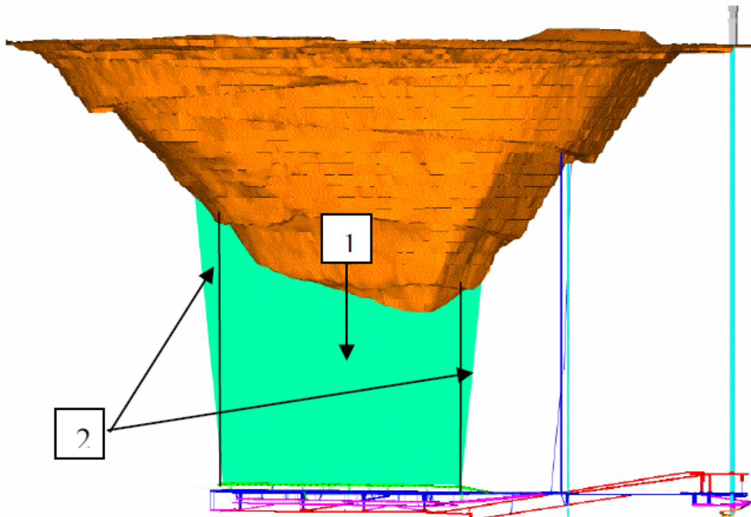
Figure 8: Ore Loss effects on the Palabora reserve from external dilution: 1 – Dilution entry, 2 – Replacement of ore by waste
