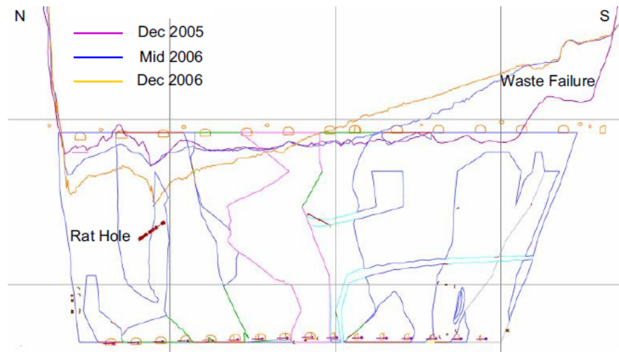
Fig.11. GEMCOM generated section showing ALS profiles with outline geology and drift positions on 53 and 63 Levels showing
