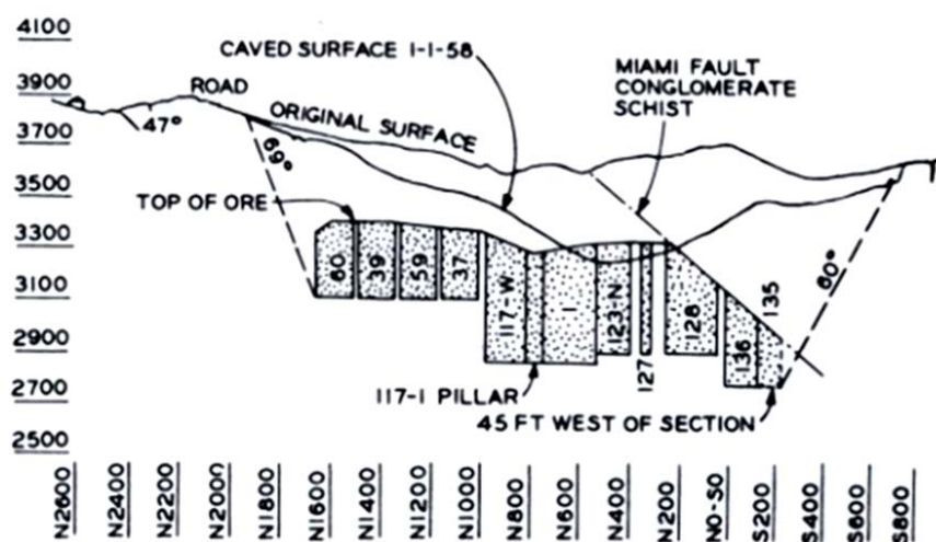
FIG. 8 E 800 section, No. 2 coordinates, showing stoped areas and subsidence, Feb. 14, 1958.
