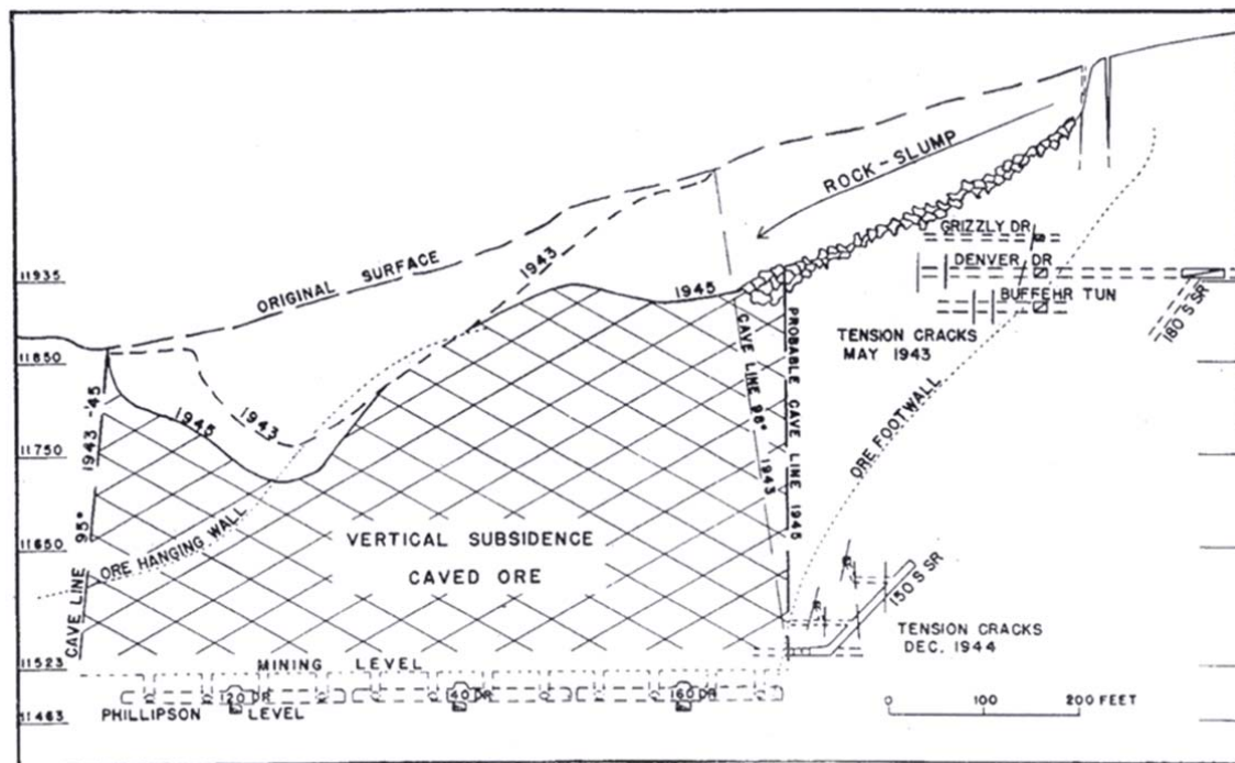
FIG. 3.—SUBSIDENCE, TENSION CRACKS AND ROCK-SLUMP IN THE CLIMAX MOLYBDENUM MINE.
