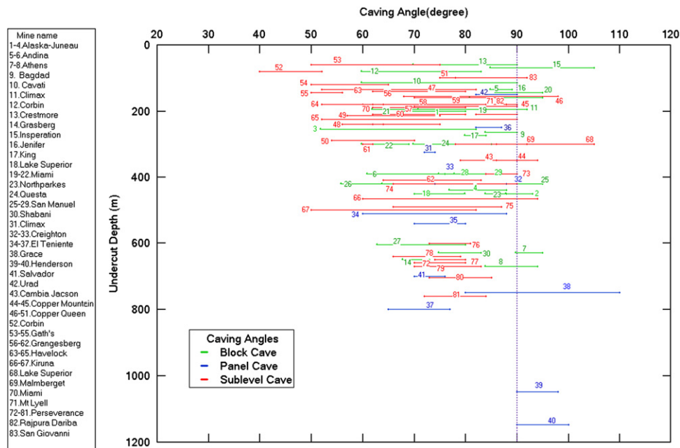
Fig. 6. Undercut depth versus caving angle for block, panel, and sub-level caving operations. Each line segment represents the range in caving angles measured from different sides of the undercut; the greater the range the higher the degree of asymmetry.
