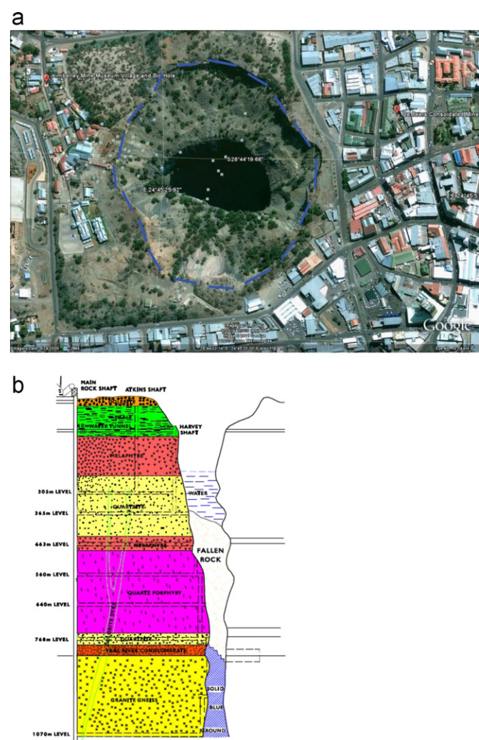
Fig. 14. Symmetric surface subsidence observed in association with a vertical kimberlite pipe-Kimberley diamond mine: (a) Google Earth satellite image, and (b) geological cross-section [11].
