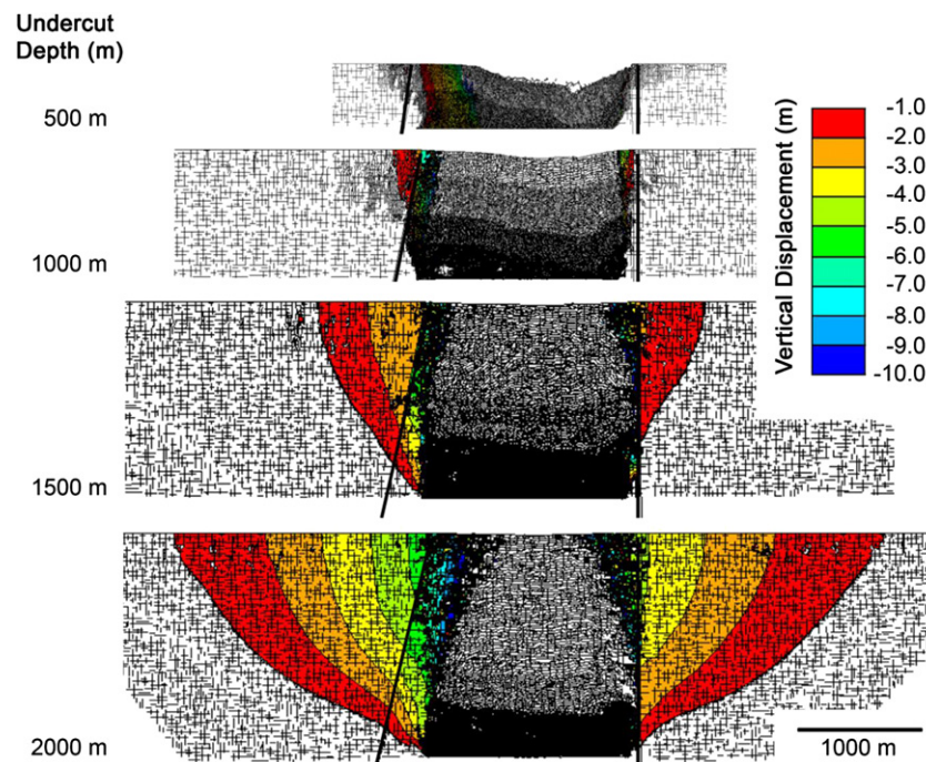
Fig. 16. ELFEN modeling results showing caving-induced brittle fracture and corresponding subsidence as a function of undercut depth. The continuous black lines to the left and right of the undercut are bounding faults.
