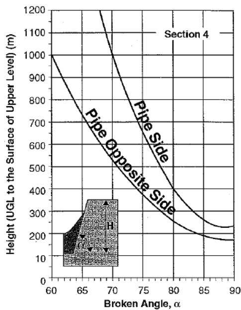
FIGURE 51.17 Variation of breakage angle with height over undercut level for section 4 (El Teniente Sur and Esmeralda sector)
