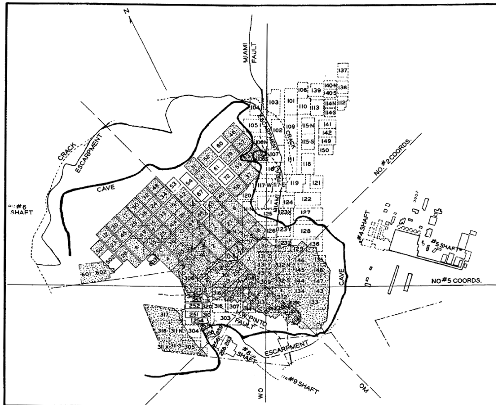
FIG. 4 Plan showing caved areas and resulting surface subsidence, July 31, 1939.
