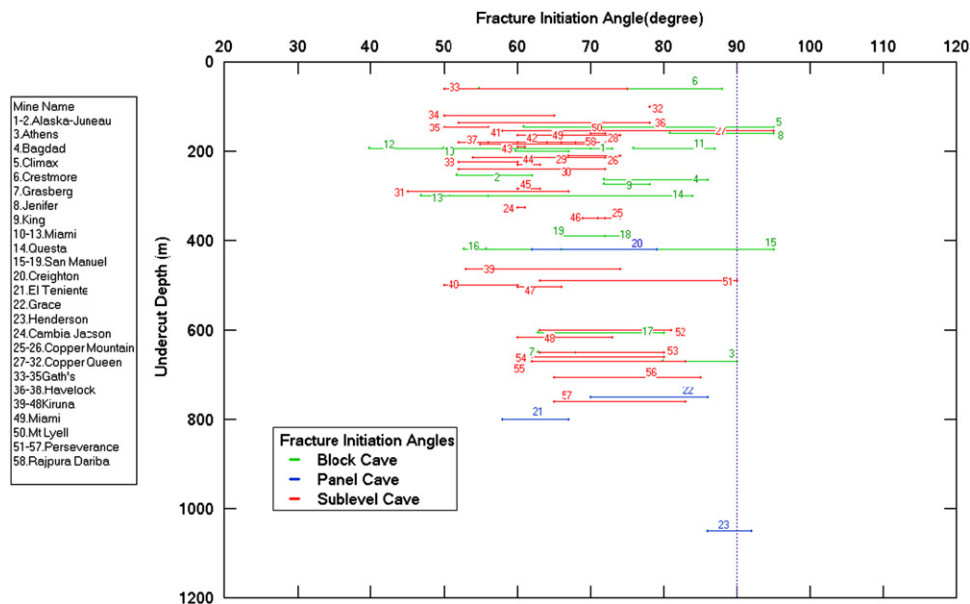
Fig. 7. Undercut depth versus fracture initiation angle for block, panel, and sub-level caving operations. Each line segment represents the range in fracture initiation angles measured from different sides of the undercut; the greater the range the higher the degree of asymmetry.
