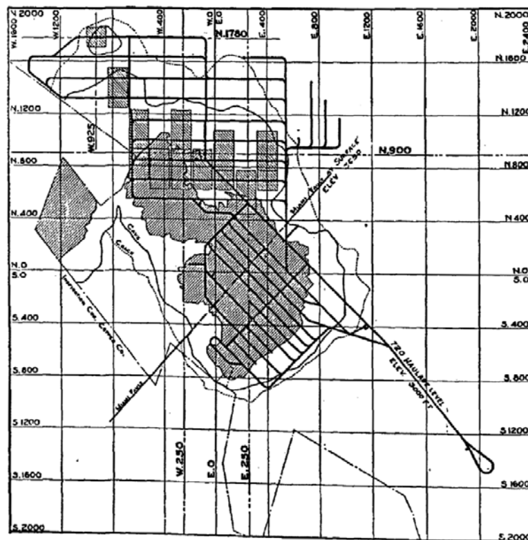
FIG. 1.—PLAN OF 720-FT. HAULAGE LEVEL, SHOWING CAVED AREAS AND RESULTING SURFACE SUBSIDENCE.
