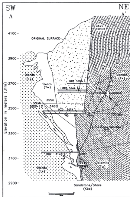
FIGURE 53.4 Geological section of EESS
