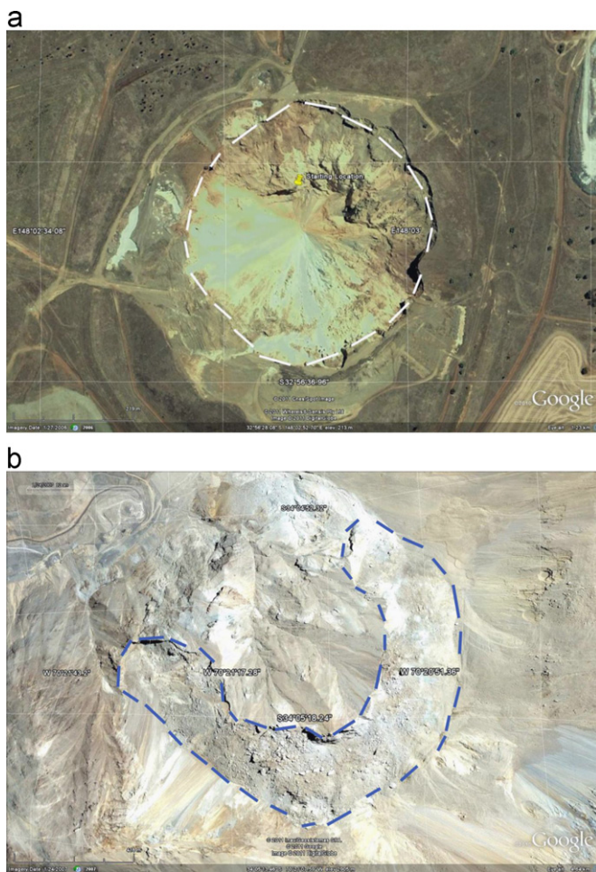
Fig. 11. Influence of topography observed visually in Google Earth satellite images: (a) flat topography (Northparkes mine, Australia), and (b) irregular topography (El Teniente mine, Chile). Surface subsidence area is marked by dashed line.
