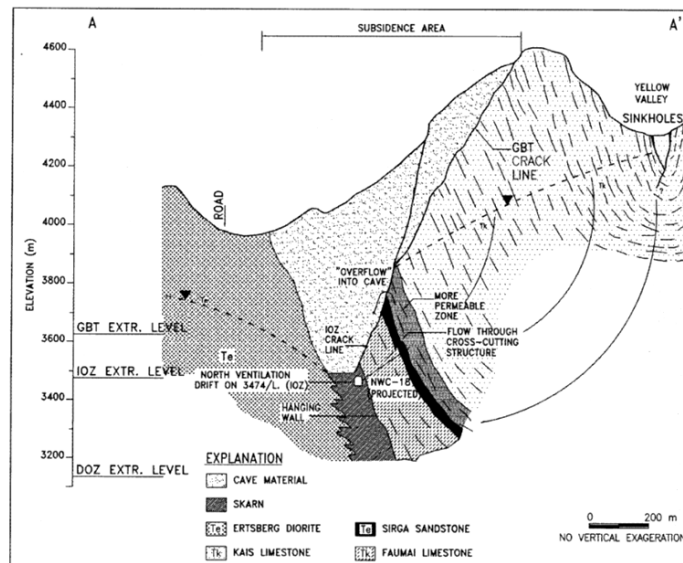
FIG 2 - Schematic long section of GBT, IOZ and DOZ.
