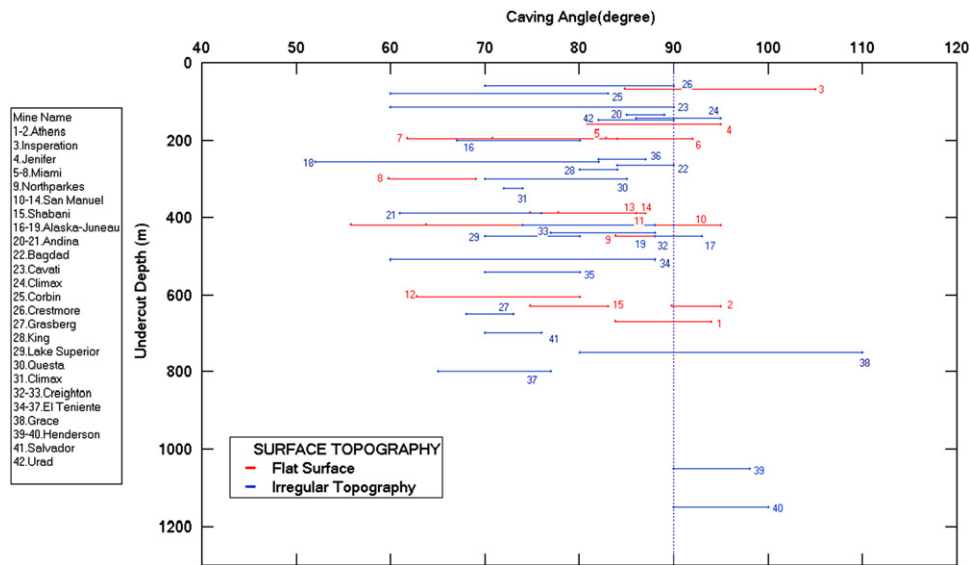
Fig. 10. Undercut depth versus caving angle for global block and panel caving operations, color coded according to the general characteristics of the surface topography. Each line segment represents the range in caving angles measured from different sides of the undercut; the greater the range the higher the degree of asymmetry. (For interpretation of the references to color in this figure caption, the reader is referred to the web version of this article.)
