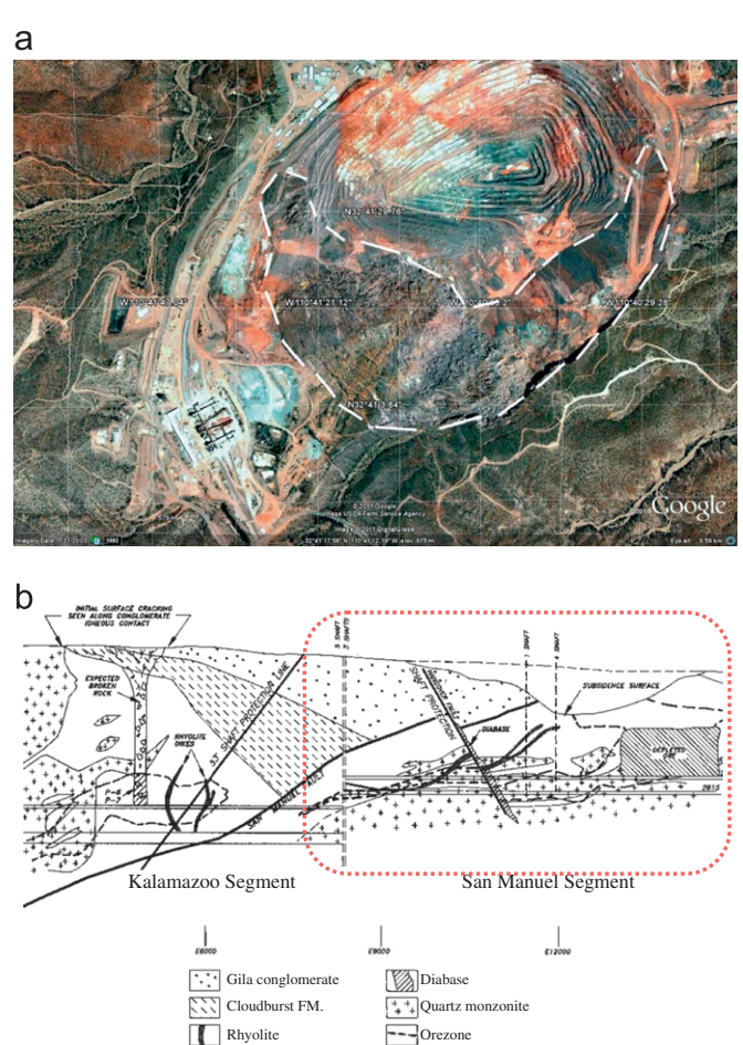
Fig. 15. Asymmetric surface subsidence observed in association with a copper porphyry ore deposit-San Manuel mine: (a) Google Earth satellite image, and (b) geological cross-section [12].
