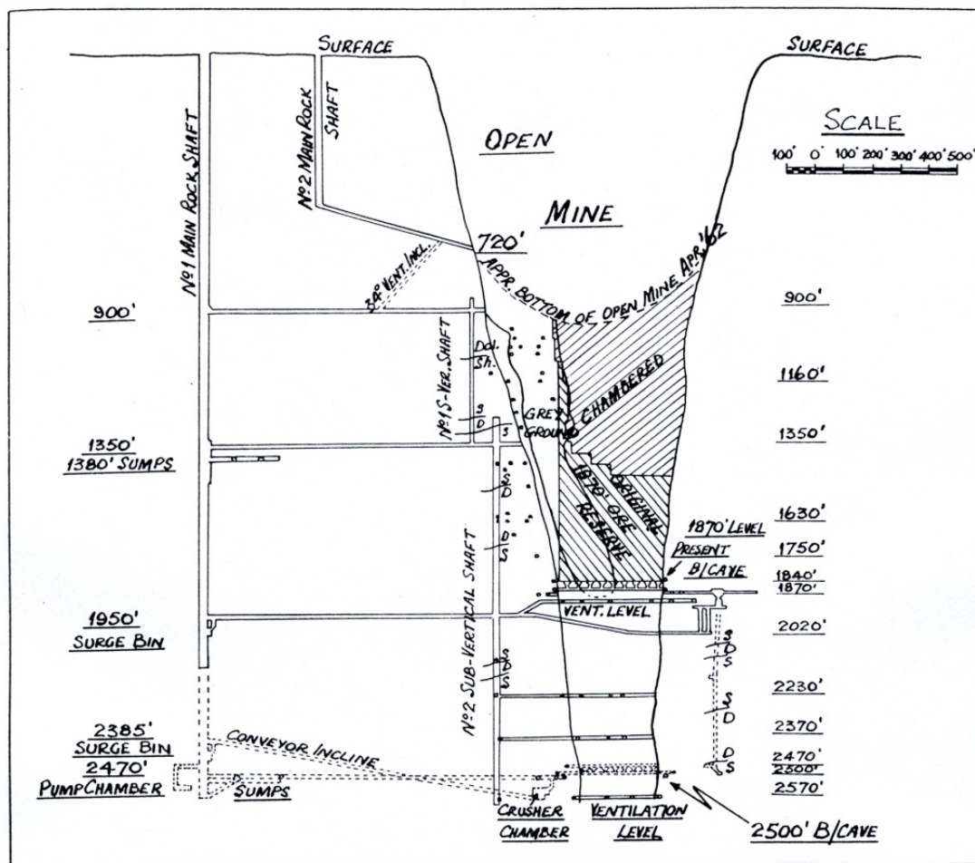
Fig. 1—Jagersfontein Mine. Diagrammatic section through Y + 31660 looking west
