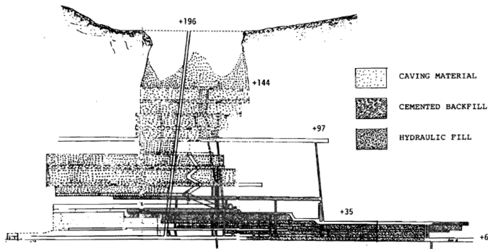
Figure 2 - Vertical longitudinal section of the "Contatto Ovest" orebody.
