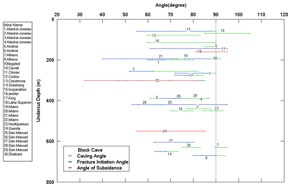
Fig. 8. Undercut depth versus caving, fracture initiation and subsidence angles for block caving operations. Each line segment represents the range in angles measured from different sides of the undercut; the greater the range the higher the degree of asymmetry.
