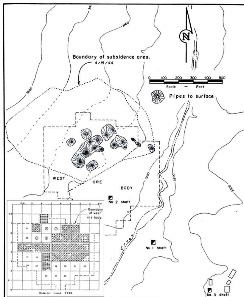
FIGURE 16. - Surface Subsidence.
