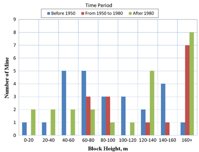
Fig. 4. Breakdown of block heights being mined for the block caving cases in the database, showing a trend towards the mining of larger blocks.
