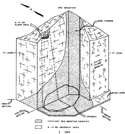
Figure 8. Position of initial surface disturbance relative to the Red Mountain igneous complex
