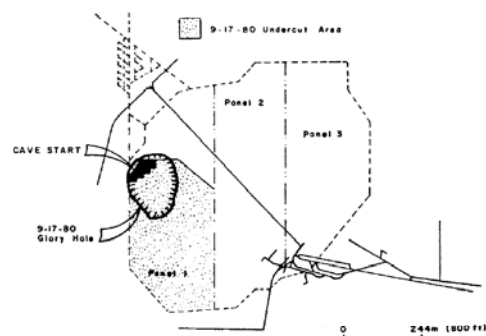
Figure 5. Position of initial surface disturbance relative to undercut area
