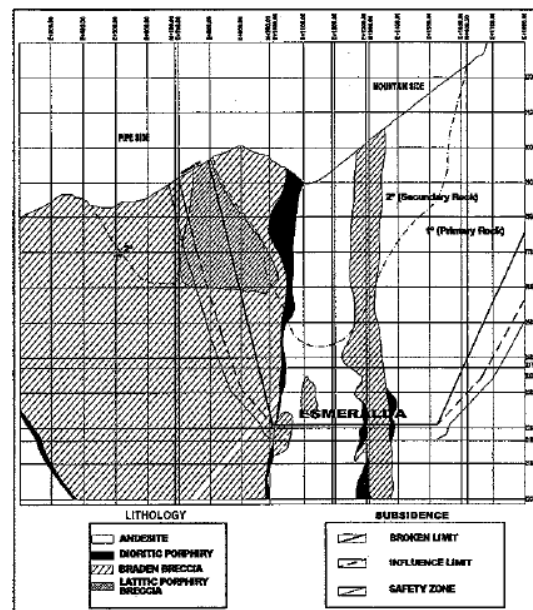
FIGURE 51.18 Southwest-northeast section through Esmeralda sector showing expected subsidence limits (defined by breakage angle and zone of influence)
