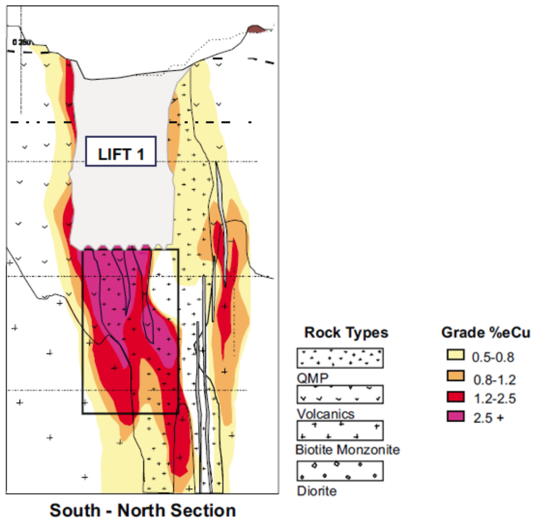
FIG 3 - E26 mine geology – Section.
