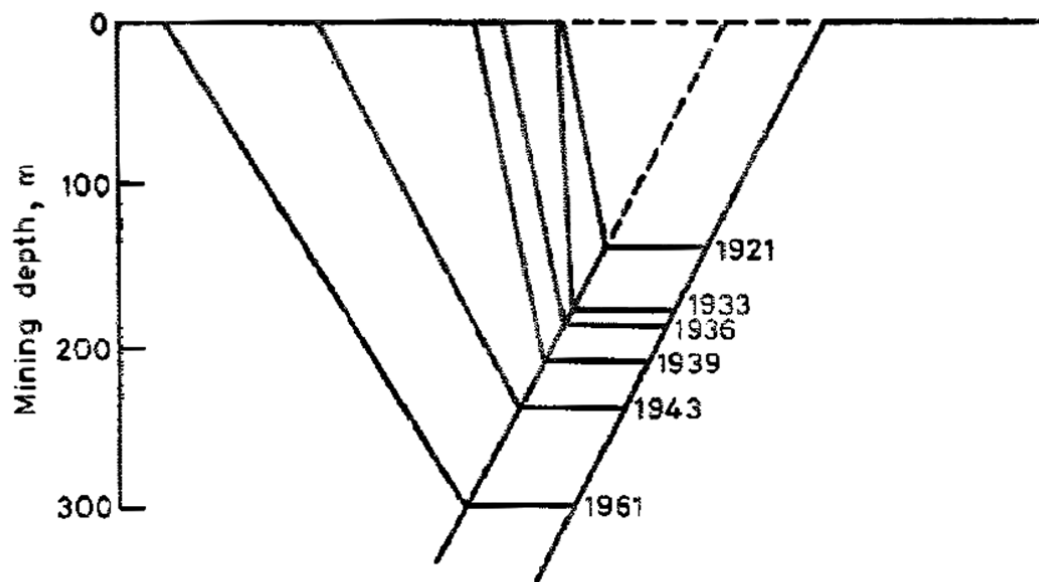
Fig. 8 Hanging-wall failure induced by caving at Grangesborg
