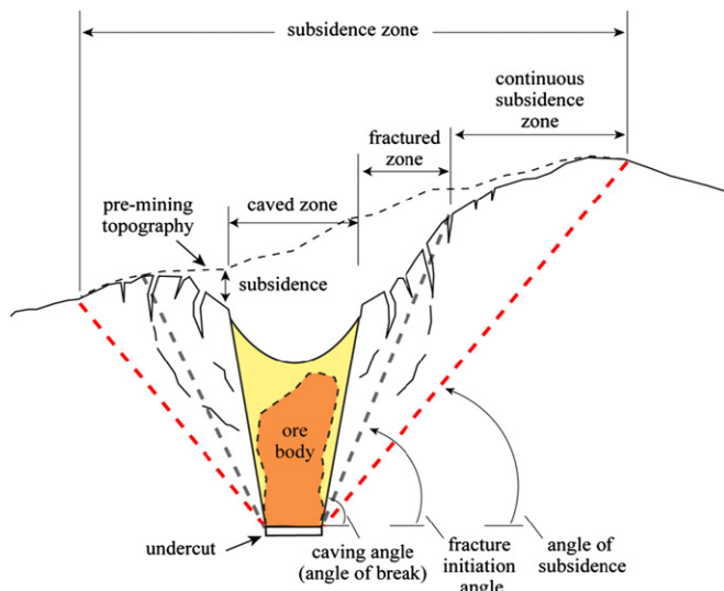
Fig. 2. Definition of block caving deformation zones as defined in [2].
