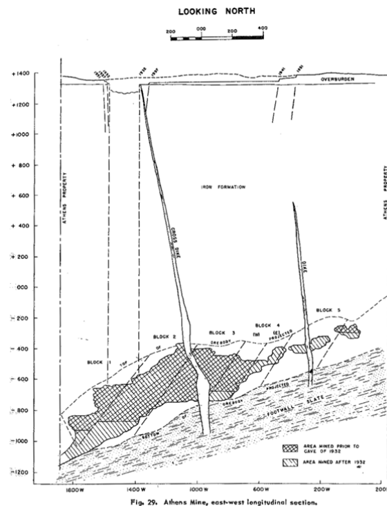
Fig. 29. Athens Mine, east-west longitudinal section.
